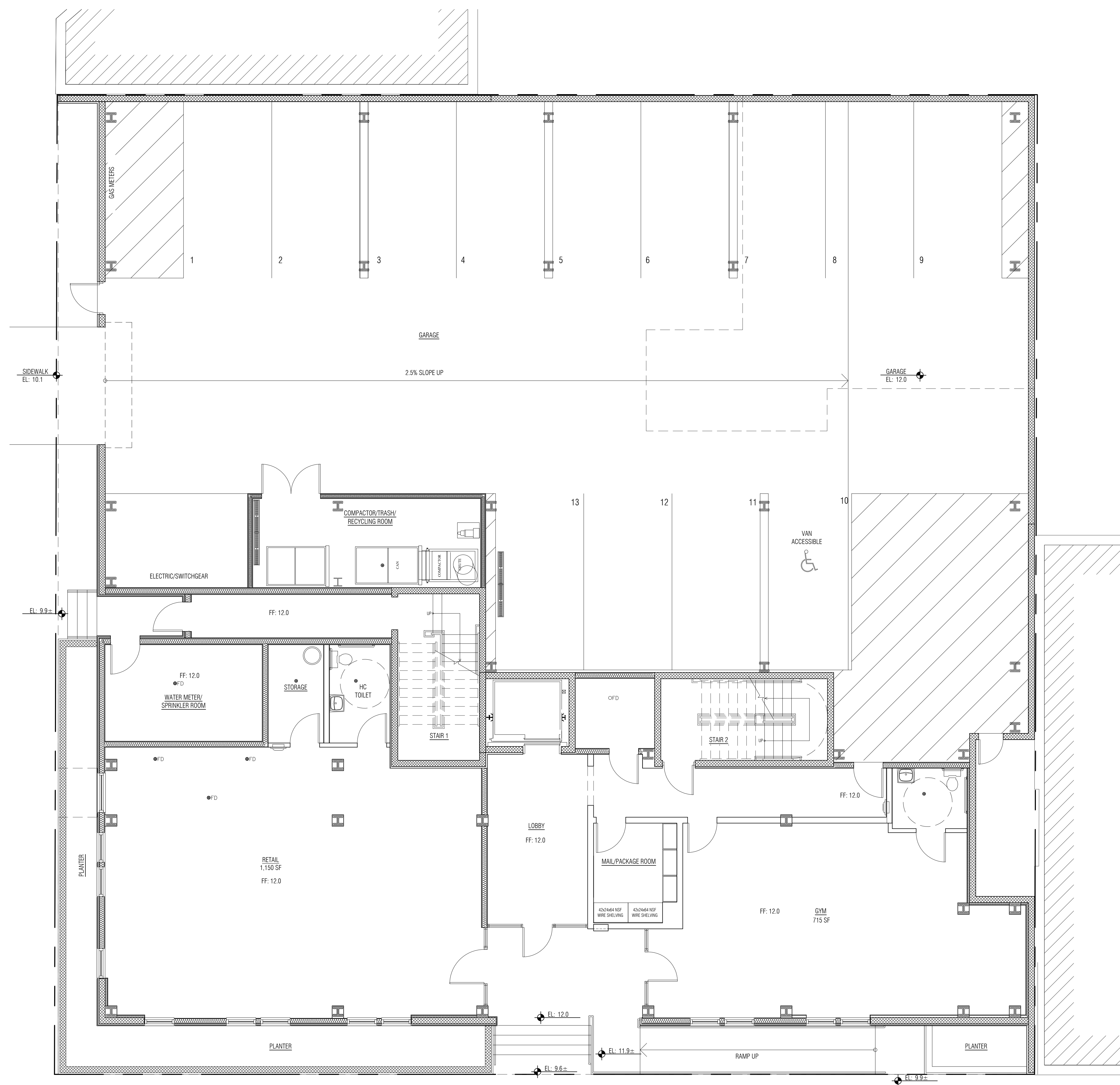
01 FIRST FLOOR - ARCHITECTURAL PLAN SCALE: 3/16" = 1'-0"
